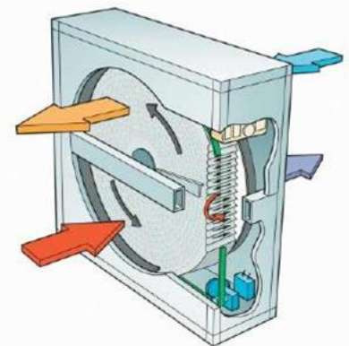
Figure 10: Heat Recover Wheel
